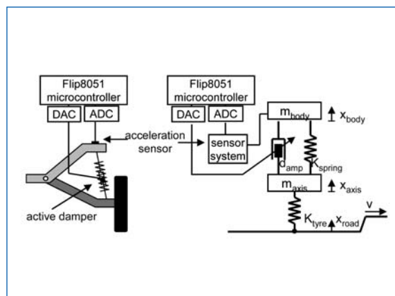
Figure 1. Active car suspension
